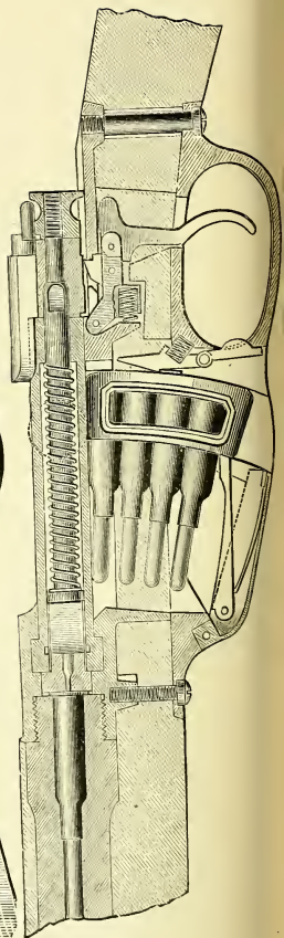
Roumanian Model Mannlicher, 1892
